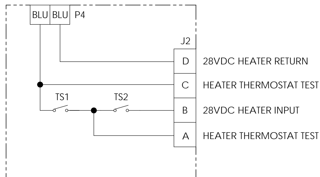
ELECTRICAL SCHEMATIC
